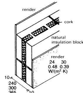
③ Natural clay insulation blocks (Bioton) 0.24 0.30 0.48 0.39 W/(m 2 ·K)
